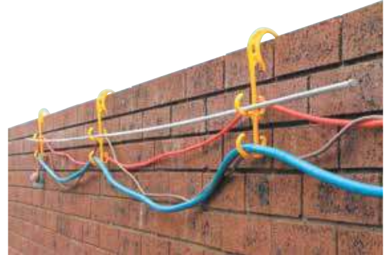
Lead Hook Stand (bucket not included)
