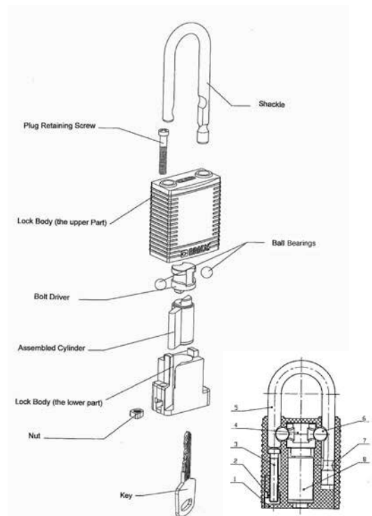
Brady Safety Plus Padlock Exploded View
